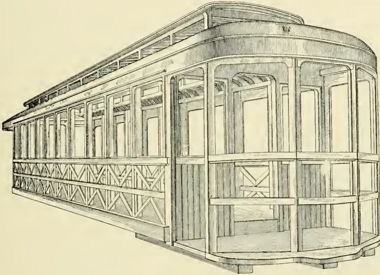
Fig. 6. Perspective View of Car Framing
